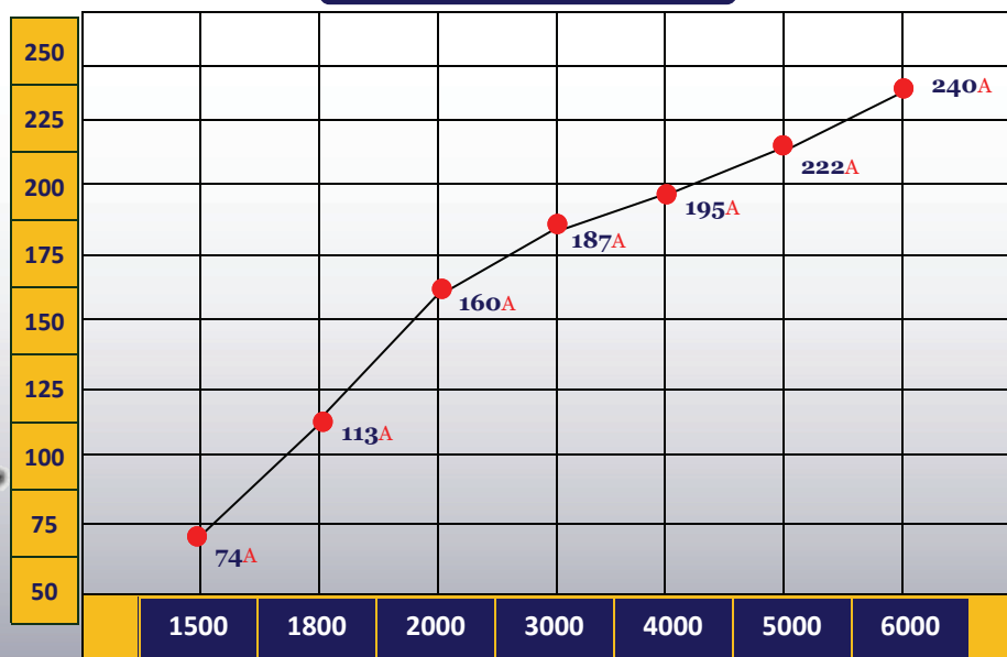
Alternator Output
