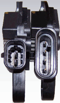
2 - Pin 4 - Pin Version Version
