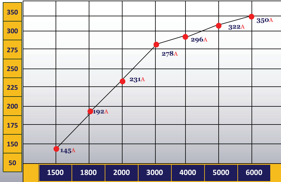
Alternator Output
