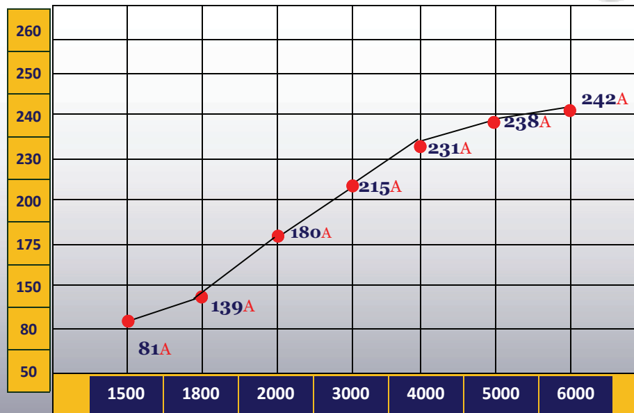
Alternator Output
