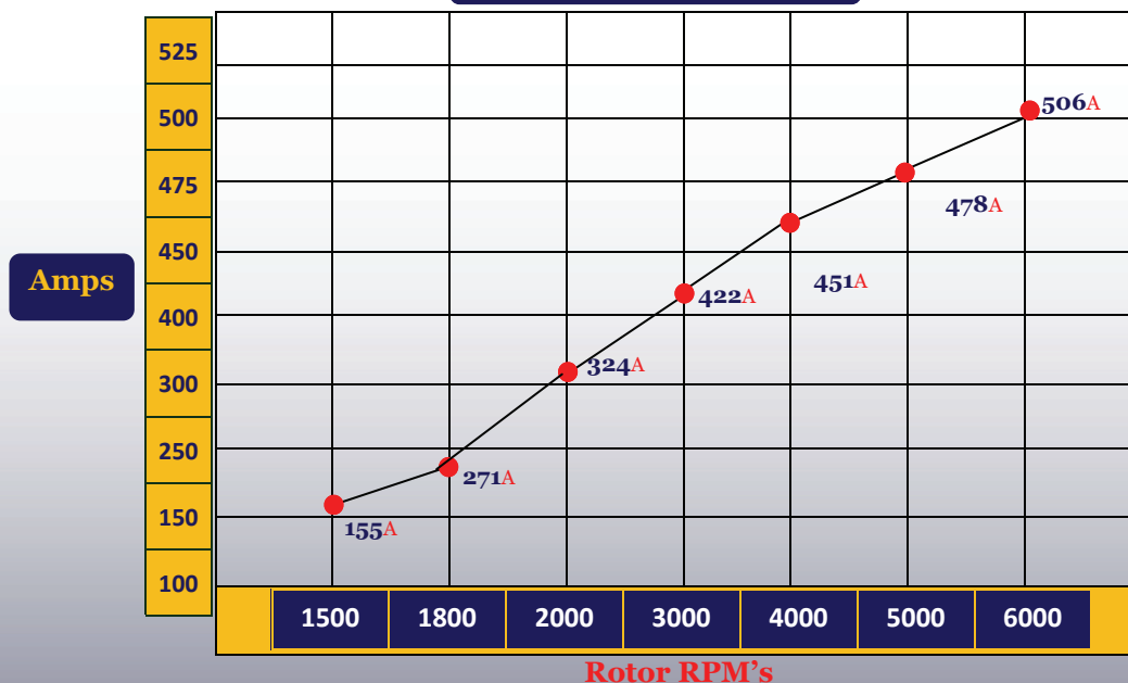
Alternator Output
