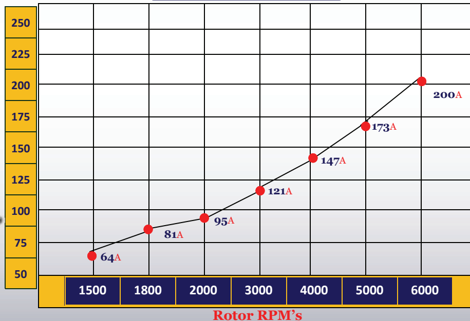
Alternator Output
