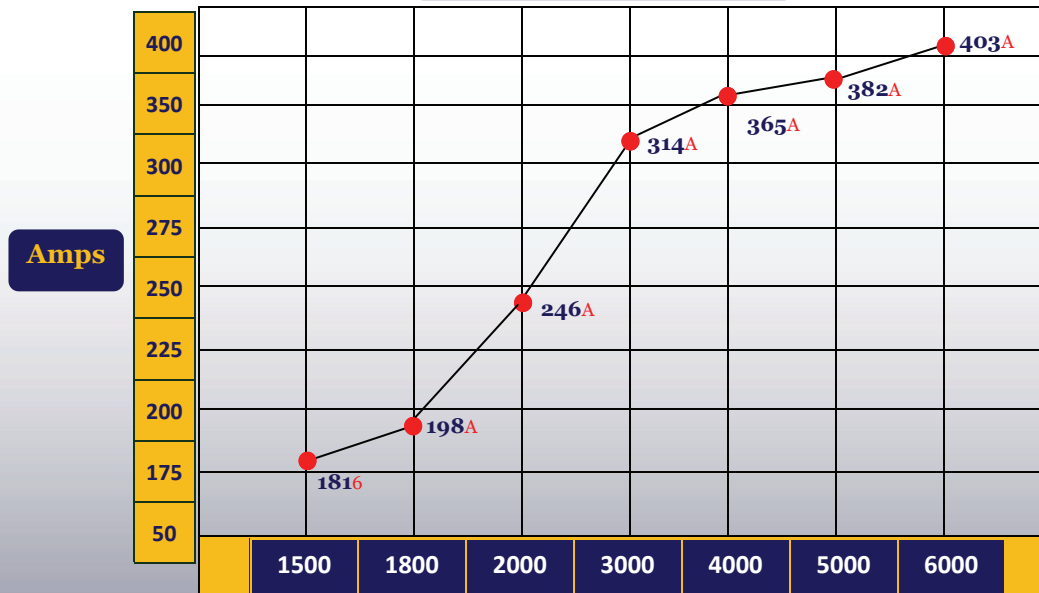
Alternator Output
