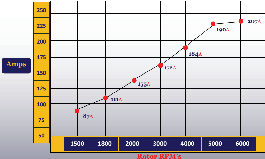
Alternator Output
