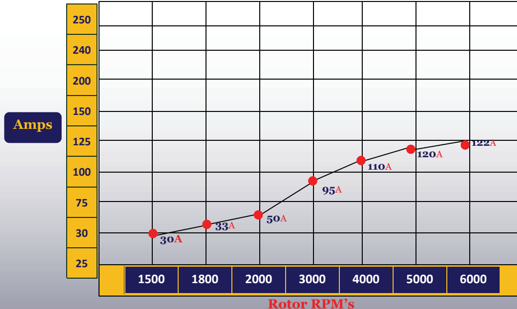
Alternator Output
