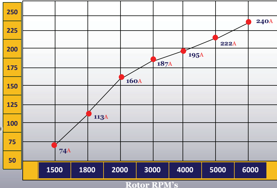
Alternator Output
