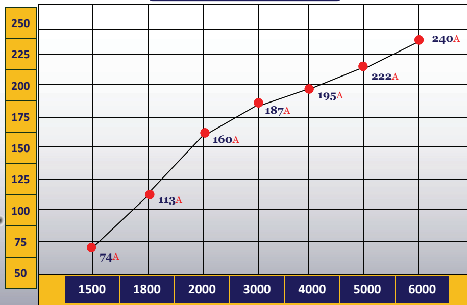
Alternator Output
