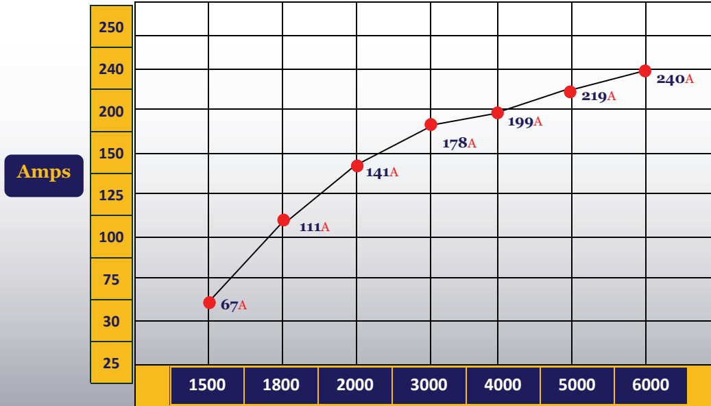
Alternator Output
